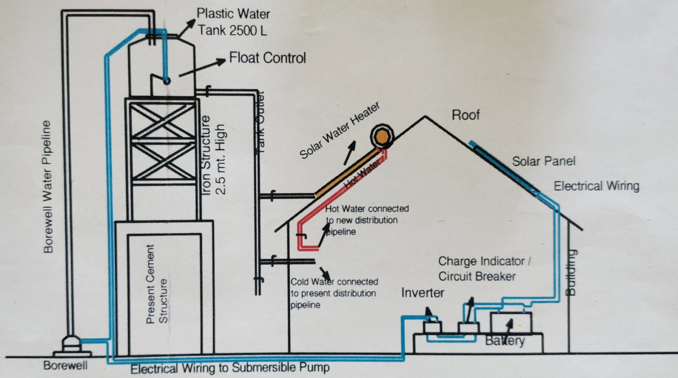
Schematic Drawing of Electrical and Plumbing installations
